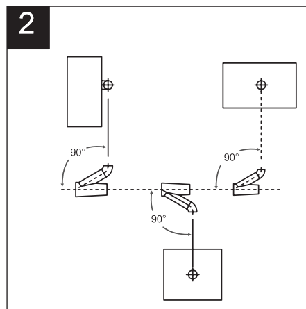
Join the 60° bends to the 30° branches to produce required 90° angle using SpeedLock joining rings. Duct end seals should be used with standard, universal and wide lock rings.
