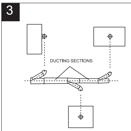
Connect the branches to intermediate ducting sections of the correct length and diameter. Adjustment to length is simplified by using a SpeedLock telescopic section.
