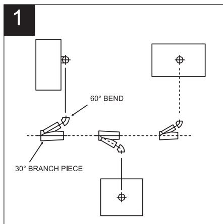
Lay out all 30° branch pieces and 60° bends on the floor in line with the hood entry points as shown.
