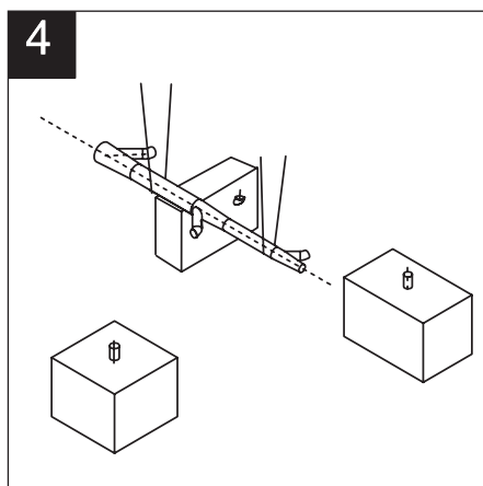
Carefully hoist the new main or sub-main assembly into position.
