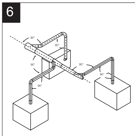
Connect risers to branch pieces. Connect main to extraction ducting system and support with SpeedLock hanging brackets.
