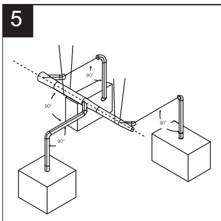
Fit machine hoods and risers; then fit another 90° bend at the top of each riser.
